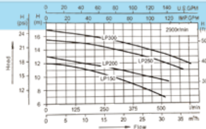
Performance Curves
