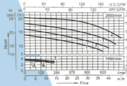
Performance Curves
