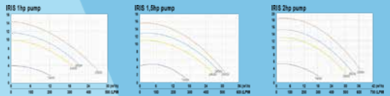
Performance Curves
