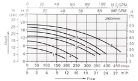
Performance Curves
