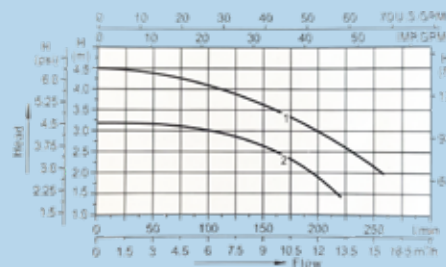
Performance Curves
