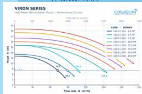
Performance Curves
