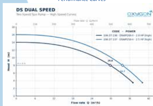
Performance Curves
