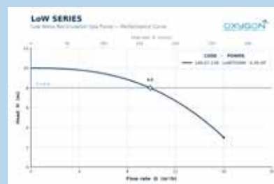
Performance Curves
