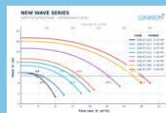
Performance Curves
