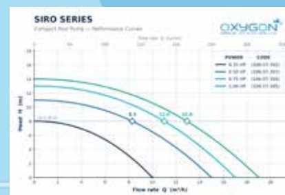
Performance Curves
