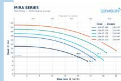
Performance Curves
