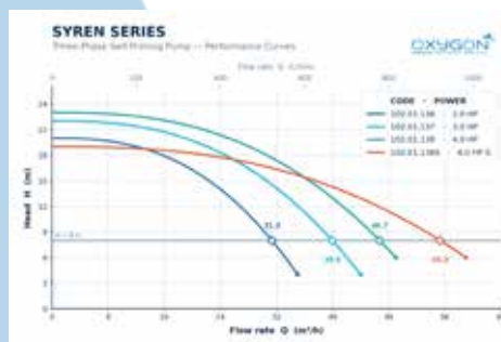
Performance Curves
